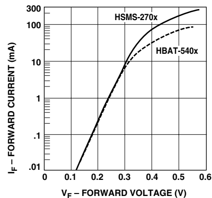
Figure 7. Forward Current vs. Forward Voltage at 25°C.
