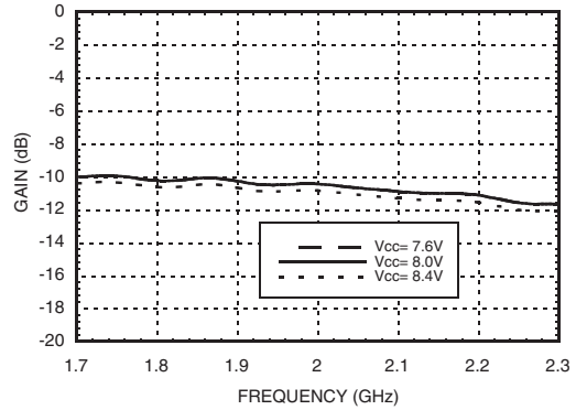
Maximum Gain vs. Supply Voltage
