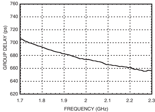
Group Delay
