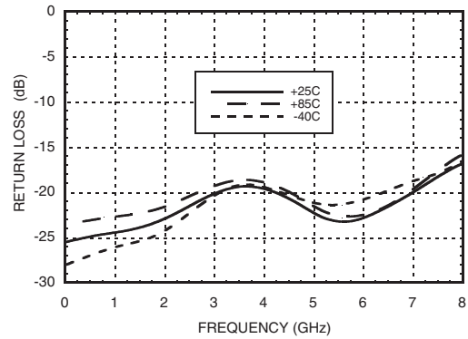
Return Loss
