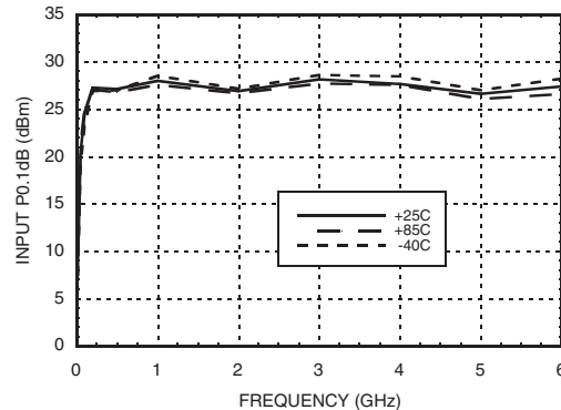
Input P0.1dB vs. Temperature
