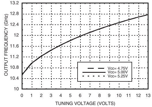
Frequency vs. Tuning Voltage, T= 25°C
