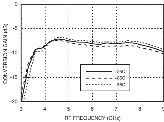
Conversion Gain vs. Temperature
