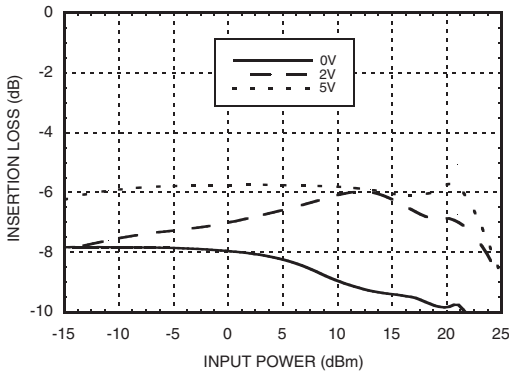
Insertion Loss vs. Pin @ 7 GHz
