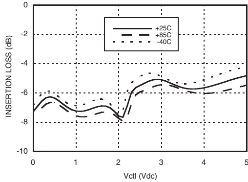
Insertion Loss vs. Control Voltage @ 11 GHz
