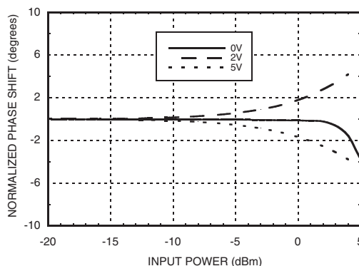
Phase Shift vs. Pin @ 15 GHz
