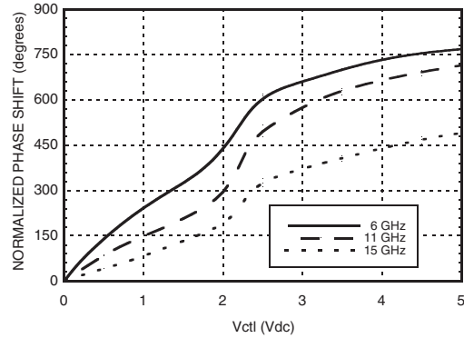
Phase Shift vs. Control Voltage
