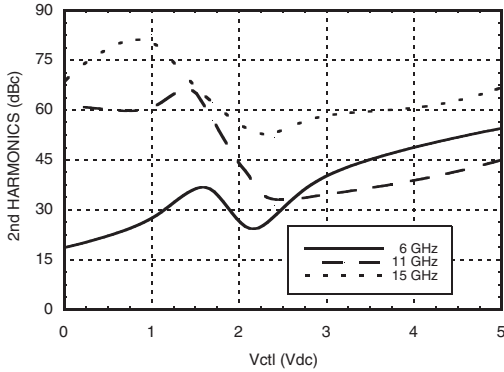
Second Harmonics vs. Control Voltage, Pin = -10 dBm
