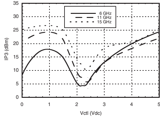
Input IP3 vs. Control Voltage
