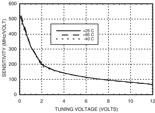
Sensitivity vs. Tuning Voltage, V_{cc1} = +5V
