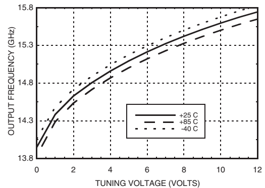
Frequency vs. Tuning Voltage, Vcc1 = +5V
