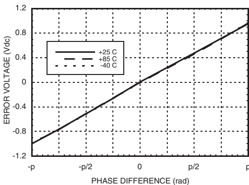
Error Voltage vs. Temperature P_{in} = 0 \text{ dBm} , F_{in} = 235 \text{ MHz}
