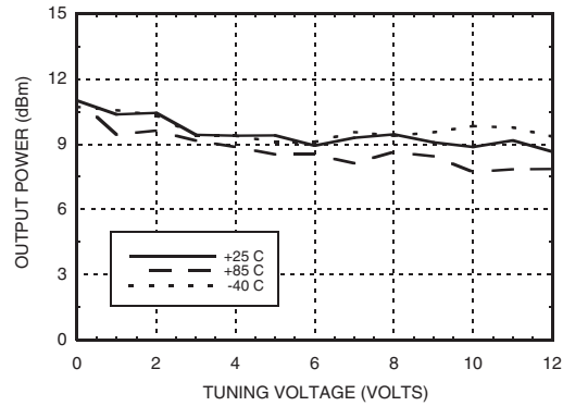
Output Power vs. Tuning Voltage, V_{cc1} = +5V
