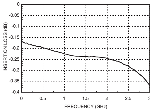
Insertion Loss, T = +25 °C
