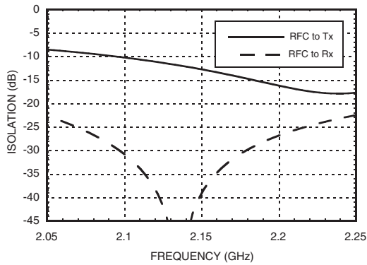
Isolation with 2140 MHz Tuning
