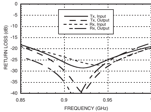
Return Loss with 915 MHz Tuning
