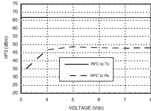
Input IP3 vs. Voltage with 915 MHz Tuning
