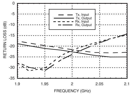
Return Loss with 2015 MHz Tuning
