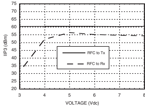
Input IP3 vs. Voltage with 220 MHz Tuning
