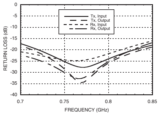
Return Loss with 785 MHz Tuning
