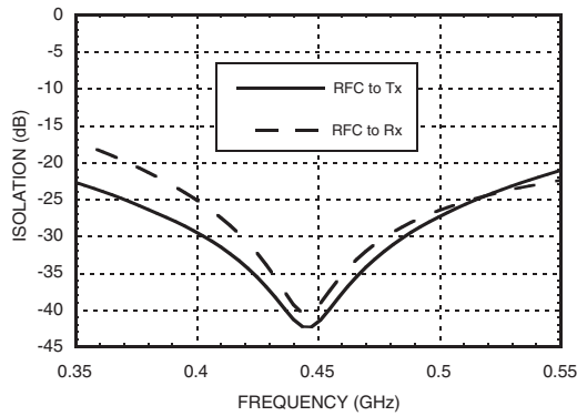
Isolation with 457 MHz Tuning
