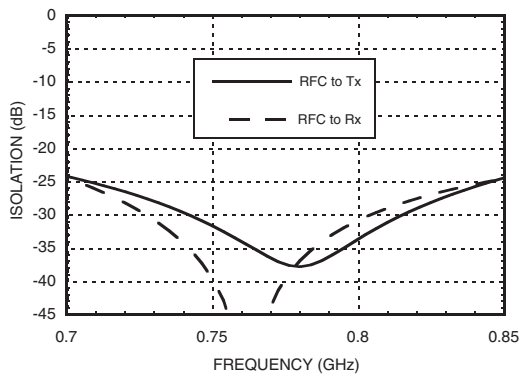
Isolation with 785 MHz Tuning
