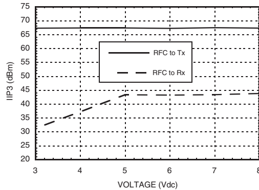
Input IP3 vs. Voltage with 2140 MHz Tuning
