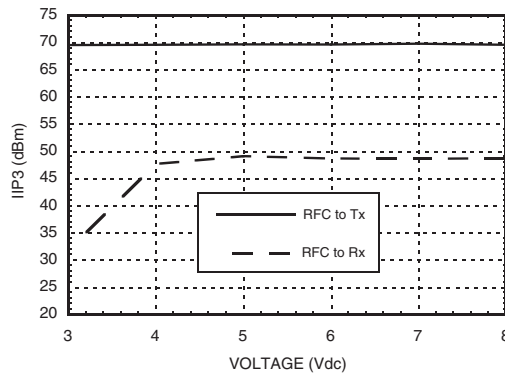
Input IP3 vs. Voltage with 785 MHz Tuning
