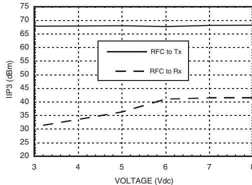
Input IP3 vs. Voltage with 1960 MHz Tuning
