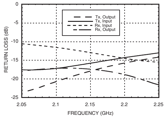
Return Loss with 2140 MHz Tuning
