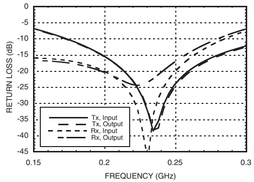
Return Loss with 220 MHz Tuning
