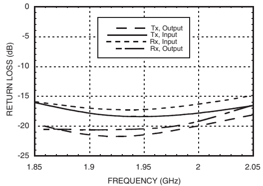
Return Loss with 1960 MHz Tuning
