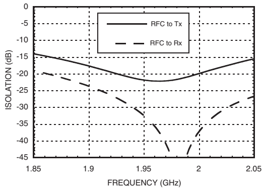
Isolation with 1960 MHz Tuning
