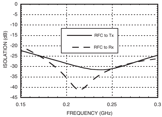
Isolation with 220 MHz Tuning
