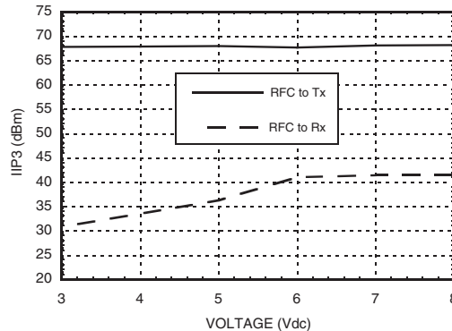
Input IP3 vs. Voltage with 2015 MHz Tuning
