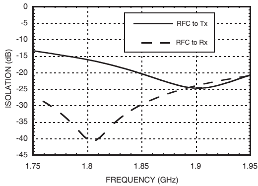
Isolation with 1843 MHz Tuning
