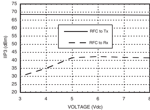
Input IP3 vs. Voltage with 1843 MHz Tuning
