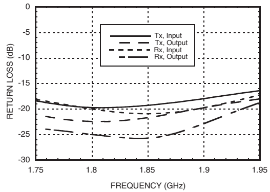
Return Loss with 1843 MHz Tuning
