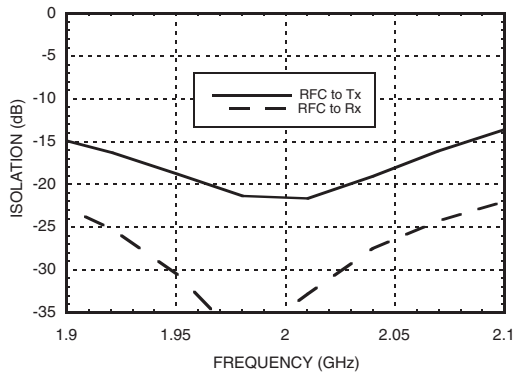
Isolation with 2015 MHz Tuning
