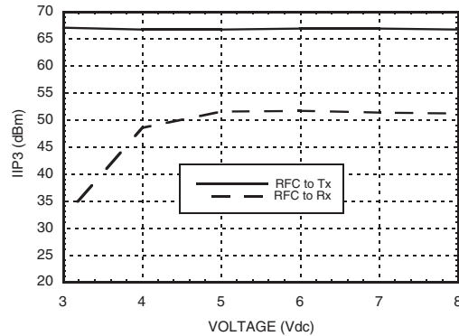
Input IP3 vs. Voltage with 457 MHz Tuning
