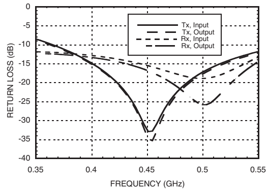
Return Loss with 457 MHz Tuning
