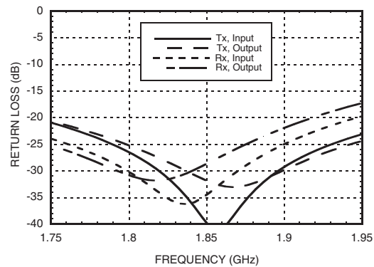
Return Loss with 1843 MHz Tuning
