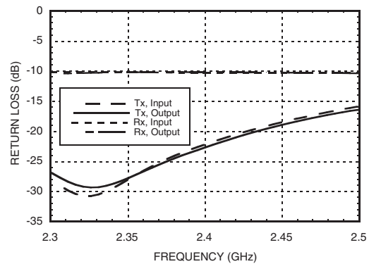
Return Loss with 2350 MHz Tuning
