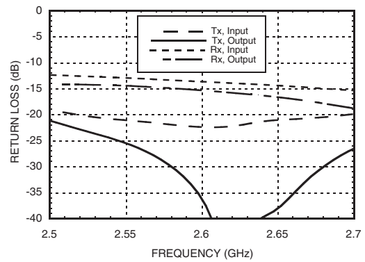
Return Loss with 2600 MHz Tuning
