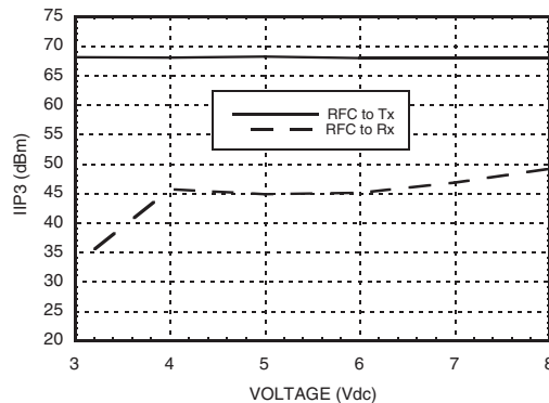
Input IP3 vs. Voltage with 2350 MHz Tuning
