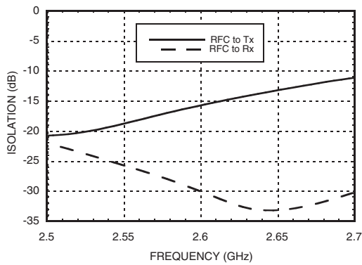
Isolation with 2600 MHz Tuning
