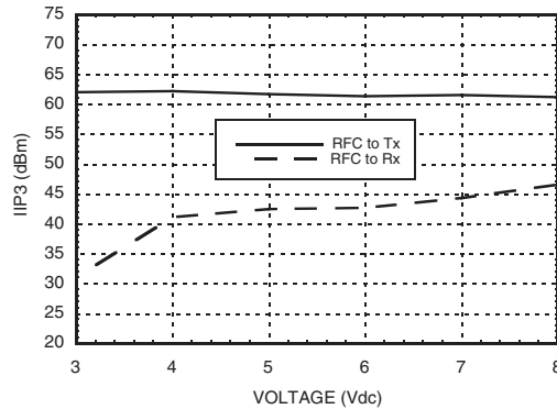
Input IP3 vs. Voltage with 2600 MHz Tuning
