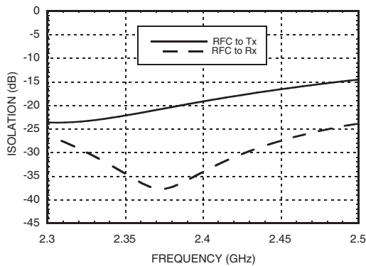
Isolation with 2350 MHz Tuning
