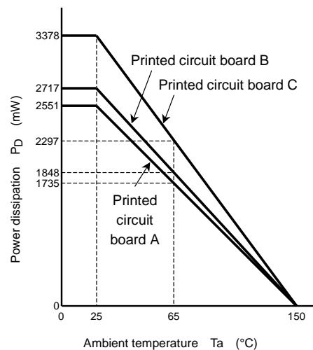
Figure 1 Characteristics of decrease in power dissipation
