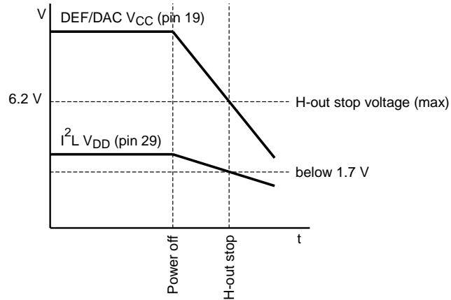
Figure (Note 4-1) V_{CC} condition at power-off
