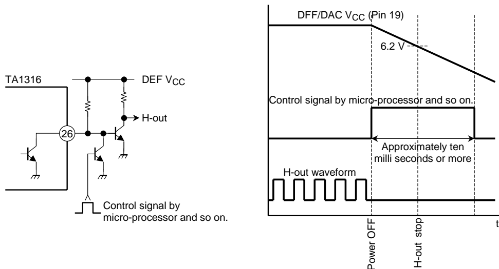
Figure (Note 4-2) Example how to stop H-out
