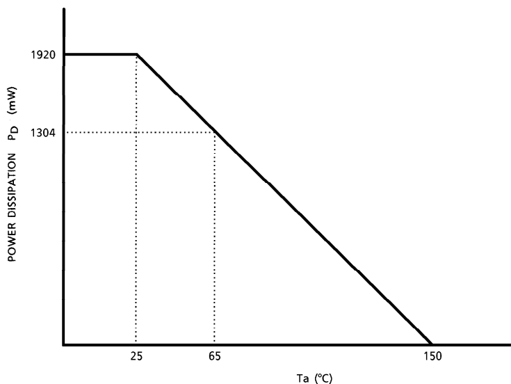
Fig. Temperature reduction curve for power dissipation
