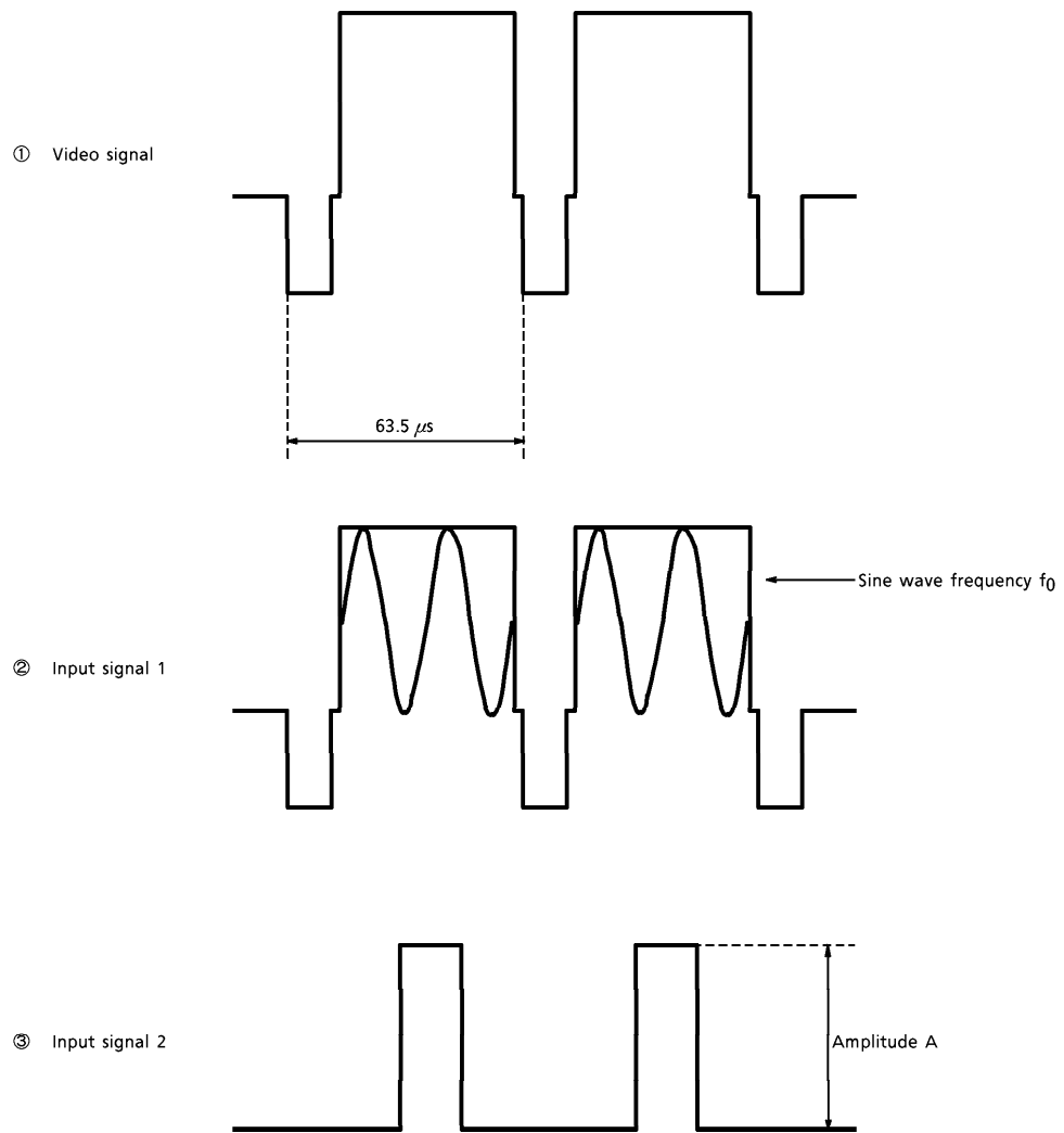
Fig.T-1 Test signals for TA1310N text stage
