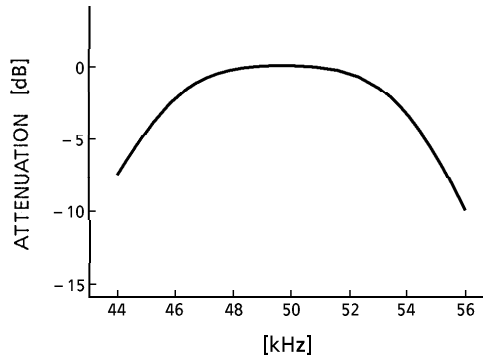
Fig.1 BPF characteristics
