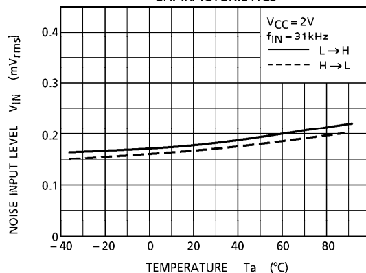
NOISE DETECTION TEMPERATURE CHARACTERISTICS
