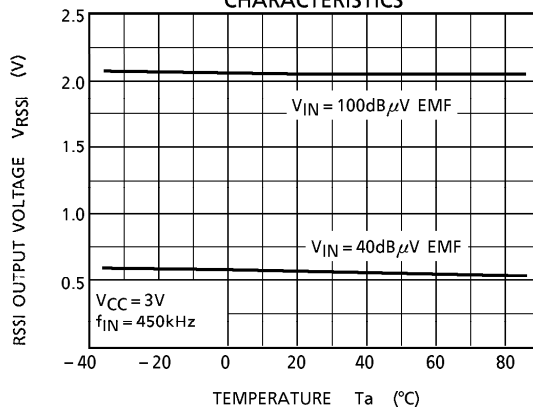
IF INPUT RSSI TEMPERATURE CHARACTERISTICS
