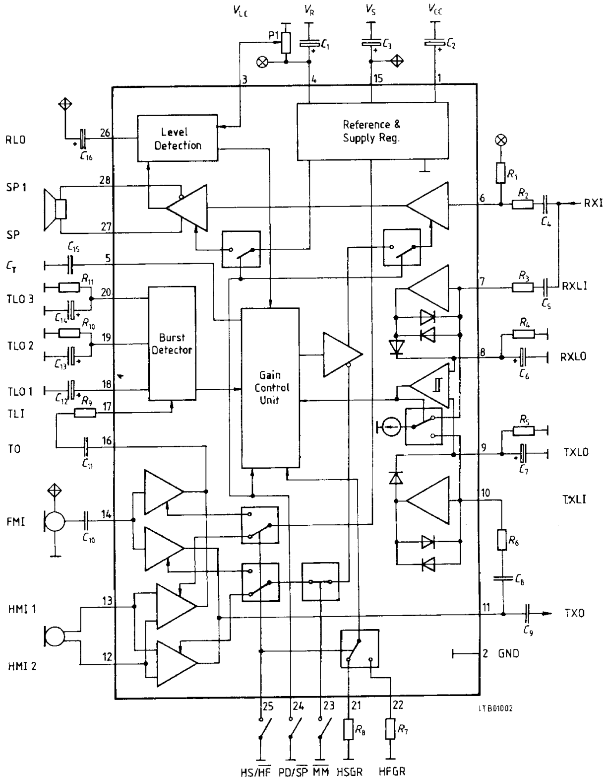
Figure 2 Block Diagram
