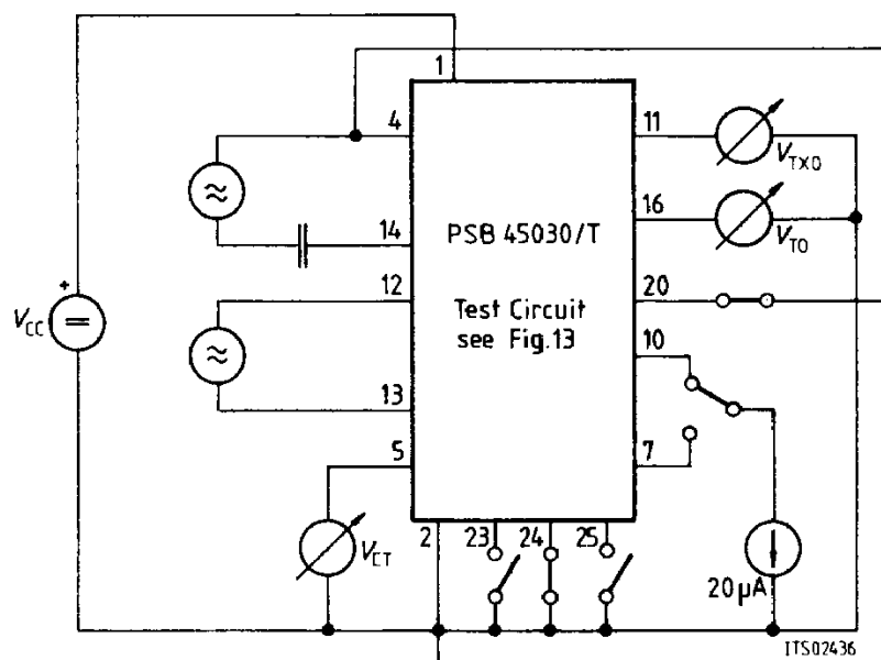
Figure 14b Test Circuit Microphone Amplifiers
