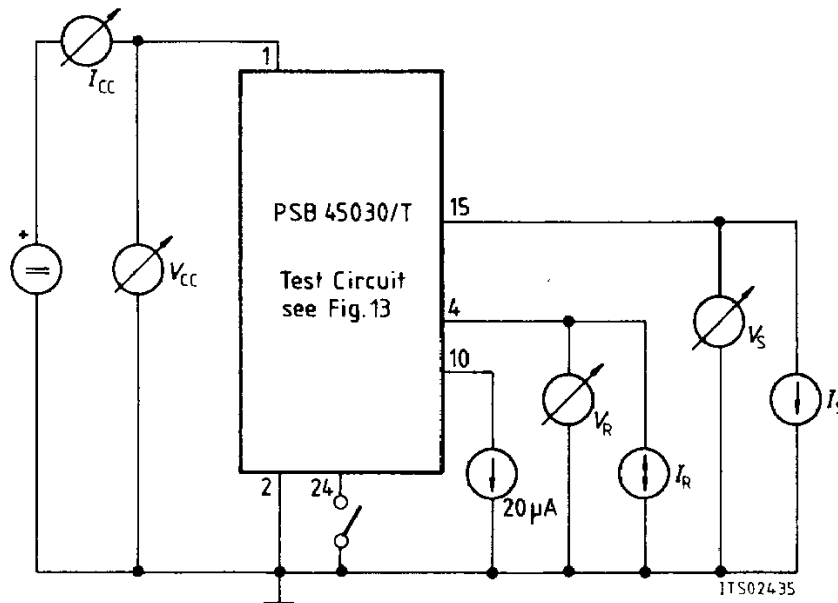
Figure 14a Test Circuit for Supply Unit
