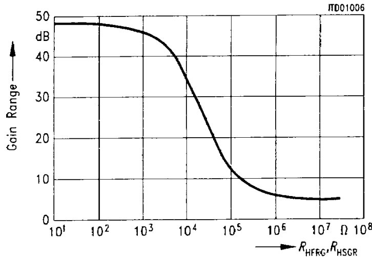
Gain Range versus R_{HFGR} and R_{HSGR}
