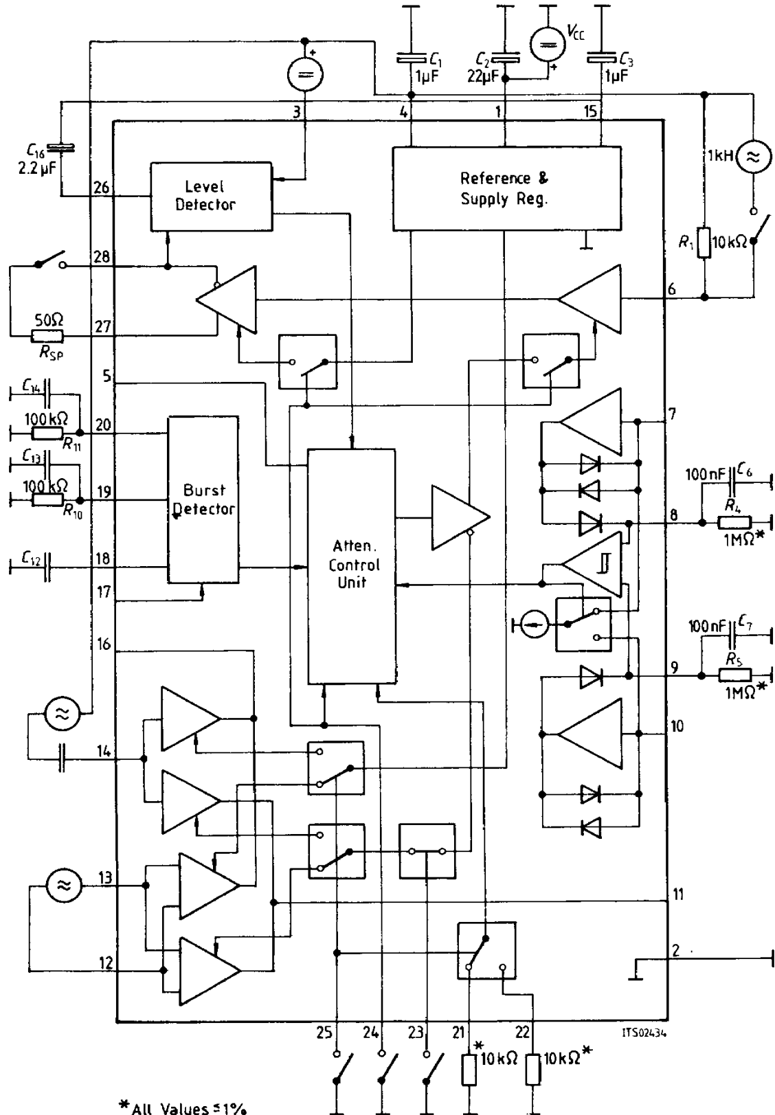
Figure 13 Basic Test Circuit
