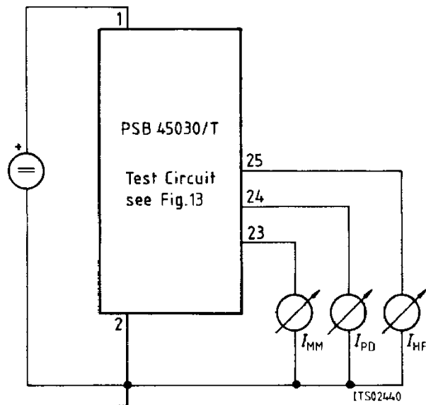
Figure 14f Test Circuit for Digital Inputs
