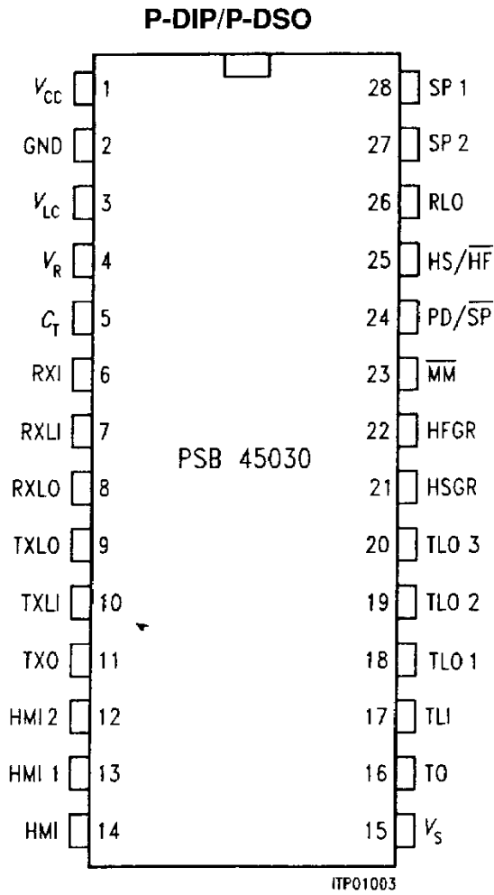
Figure 1 Pin Configuration (top view)
