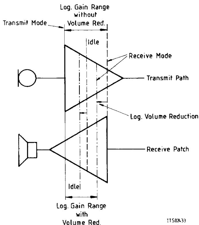
Figure 11 Principal Operation
