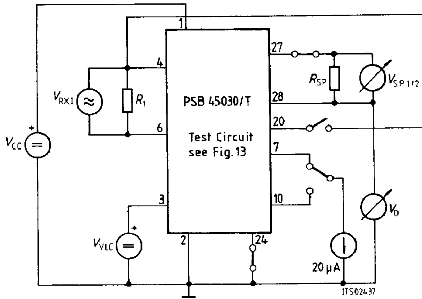
Test Circuit for Receive Amplifier with Volume Control
