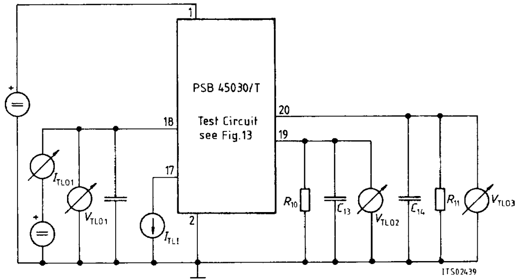
Figure 14e Test Circuit for Burst Detector
