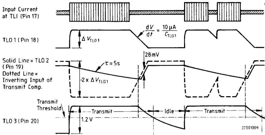
Figure 10 Burst Detector Voltages
