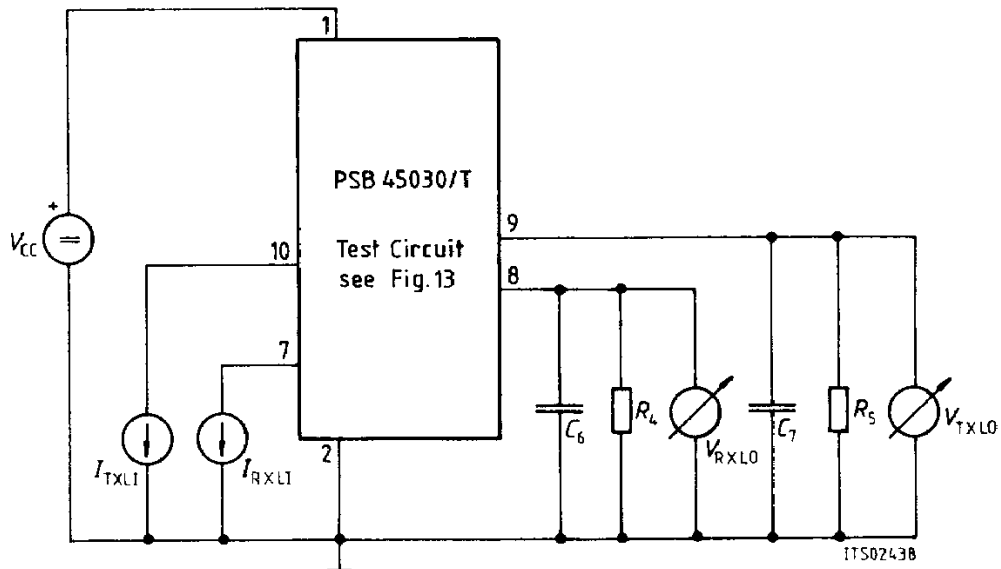
Test Circuit for Level Detectors
