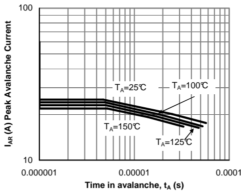
Figure 9: Single Pulse Avalanche capability (Note C)
