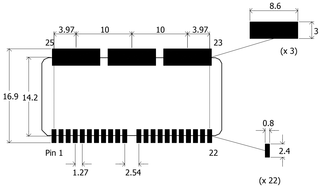
Figure 30. Recommended PCB Pad Sizes
