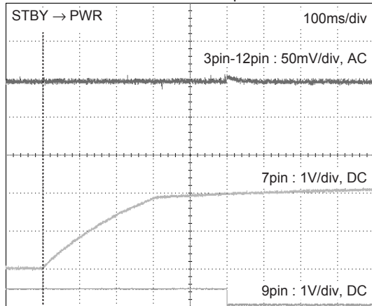
BTL mode: Turn-on transient response characteristic
