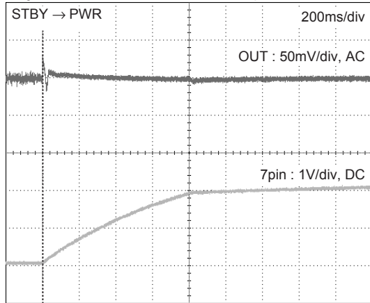
Single ended mode : Turn-on transient response characteristic
