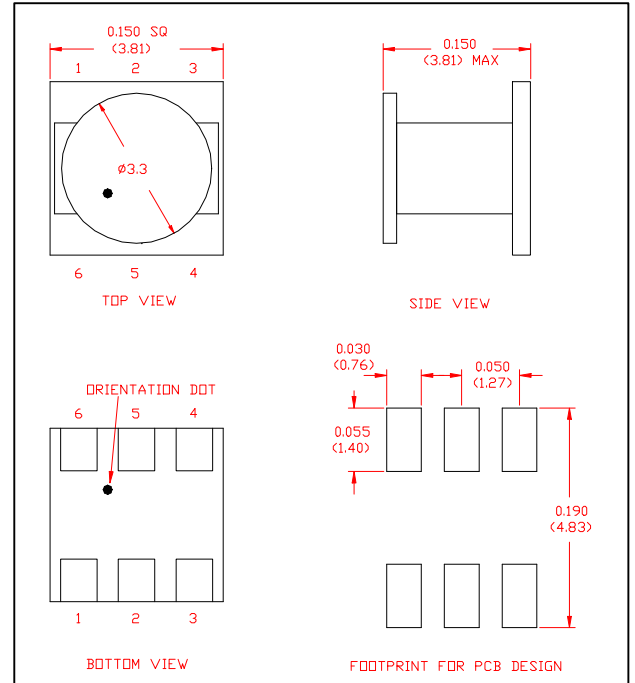
SM-156 Package
