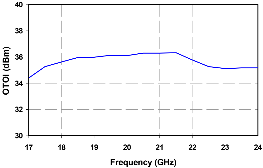
TGA2522-SM
