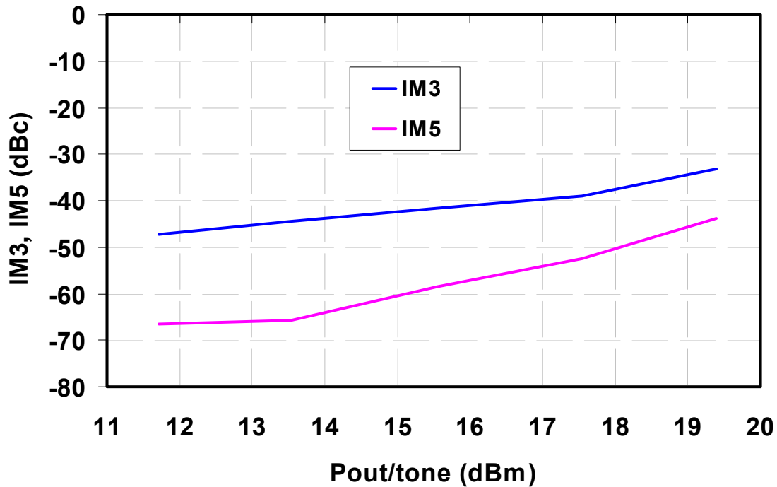
TGA2522-SM
