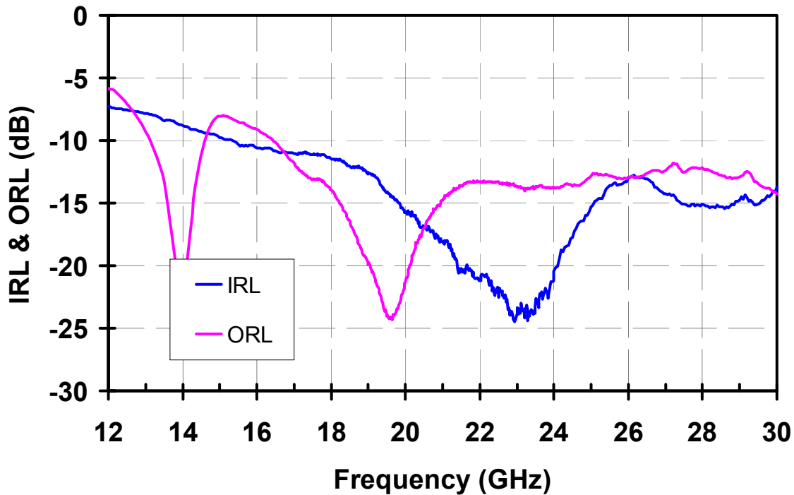
TGA2522-SM
