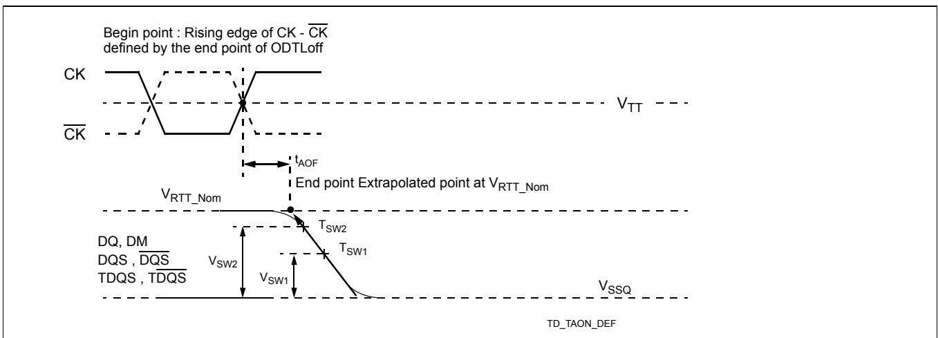
Figure 16. Definition of t_{\text{AOF}}
