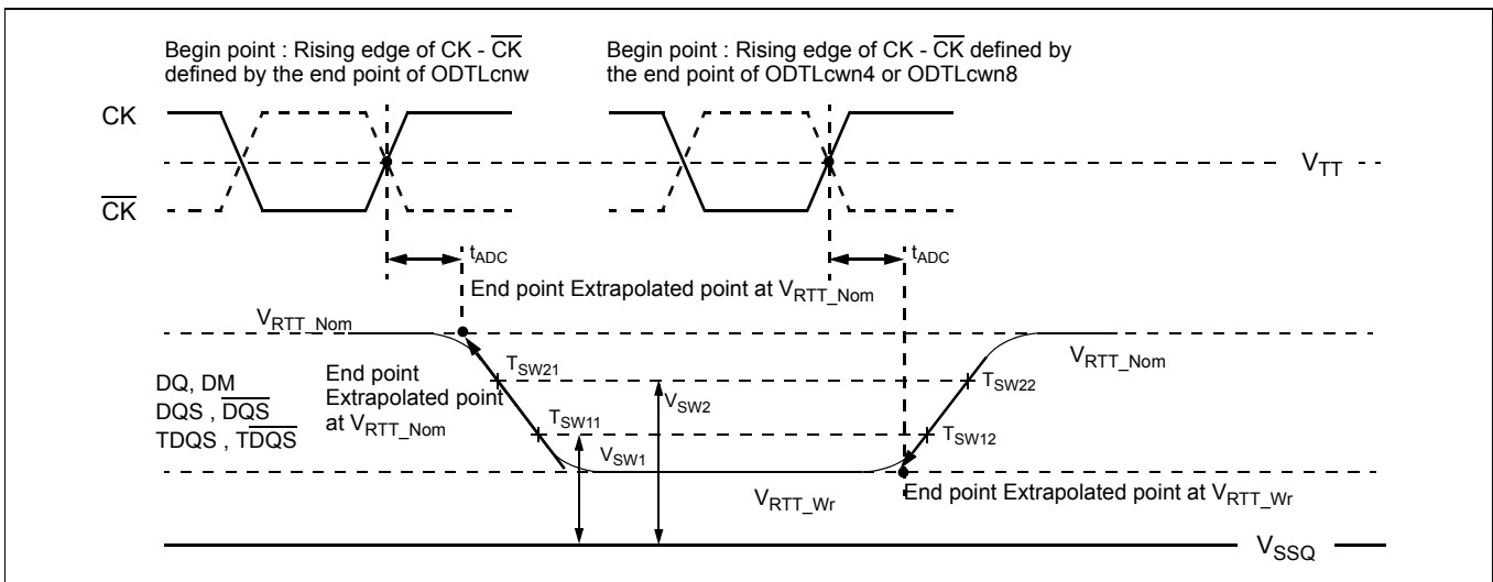
Figure 18. Definition of t_{\text{ADC}}
