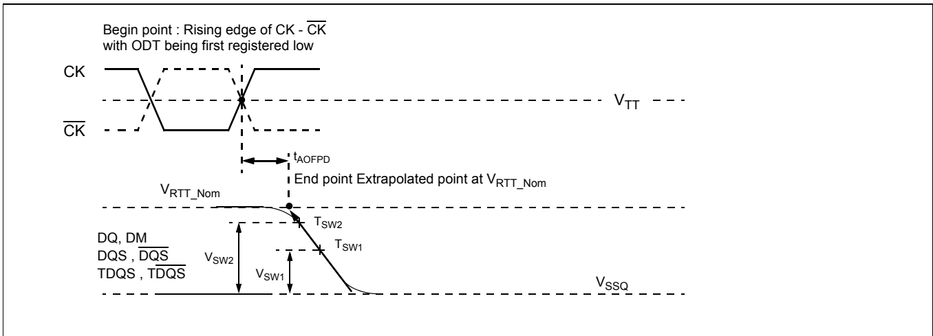
Figure 17. Definition of t_{\text{AOFPD}}
