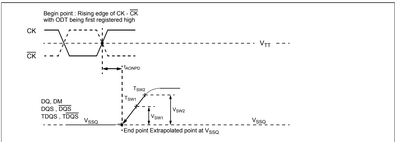
Figure 15. Definition of t_{\text{AONPD}}
