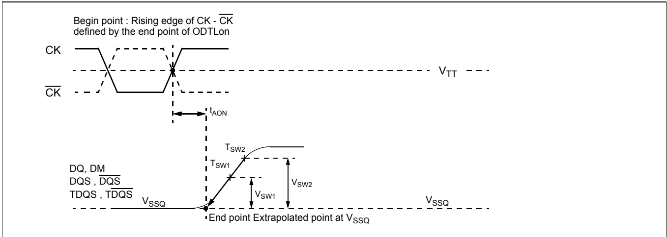
Figure 14. Definition of t_{\text{AON}}
