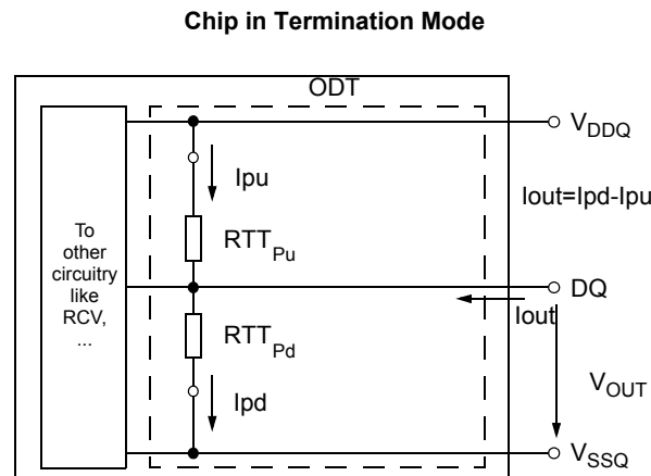
Figure 12. On-Die Termination : Definition of Voltages and Currents
