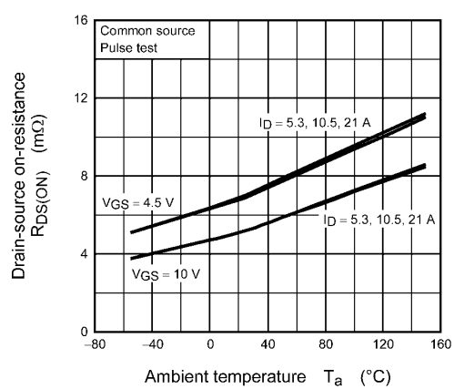
Fig. 8.6 R_{DS(ON)} - T_a
