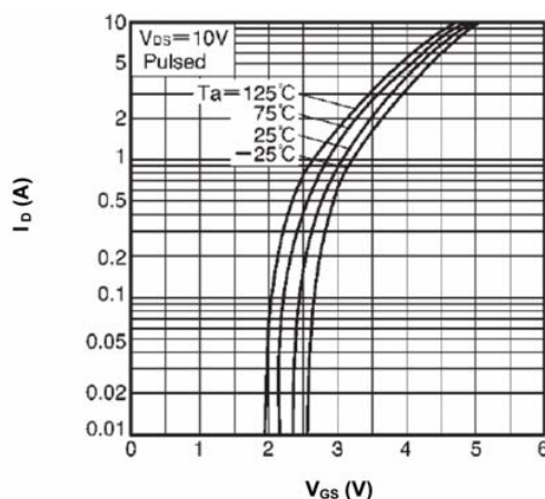
Fig 2. Transfer Characteristics
