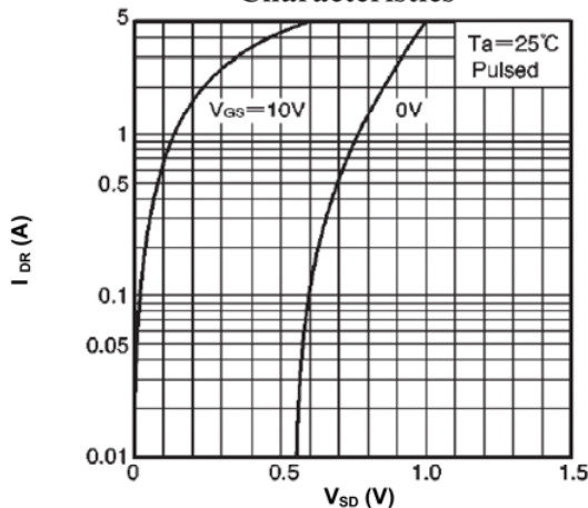
Fig 10. Reverse Drain Current vs. Source-Drain Voltage (II)
