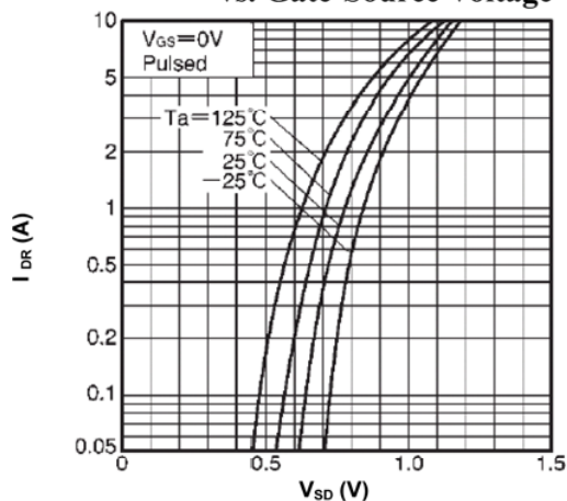
Fig 9. Reverse Drain Current vs. Source-Drain Voltage (I)
