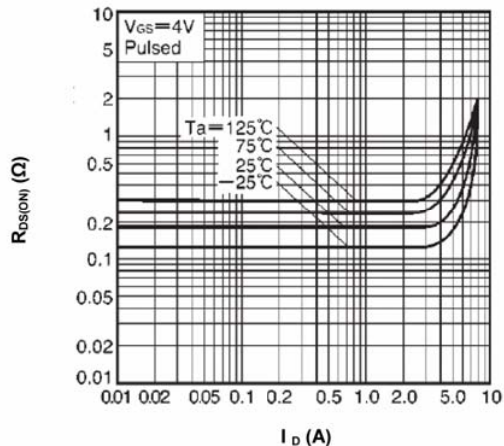
Fig 6. On-Resistance vs. Drain Current (II)
