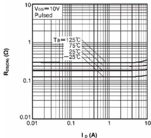
Fig 5. On-Resistance vs. Drain Current (I)
