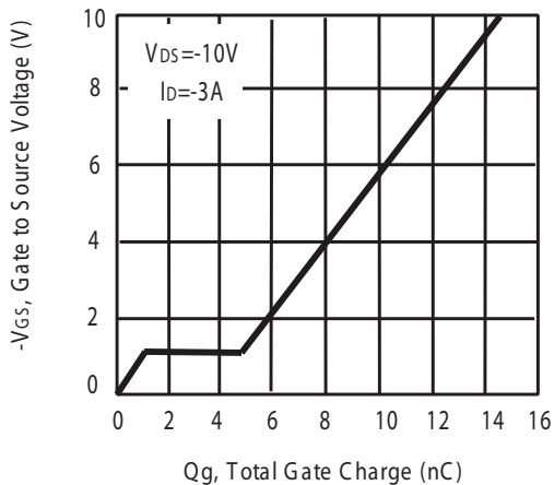
Figure 9. Gate Charge
