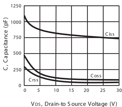
Figure 3. Capacitance
