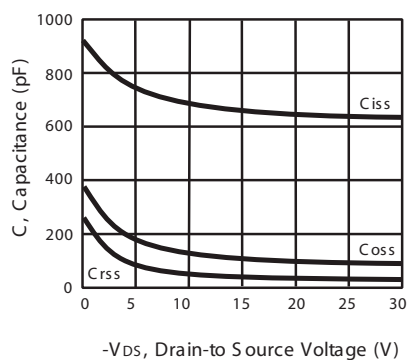
Figure 3. Capacitance
