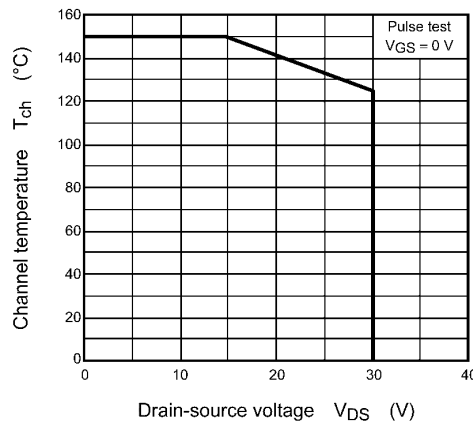
Fig. 8.17 T_{ch} - V_{DS} (Guaranteed Maximum)
