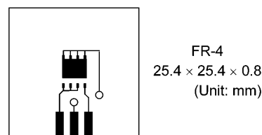
Fig. 5.2 Device Mounted on a Glass-Epoxy Board (b)
