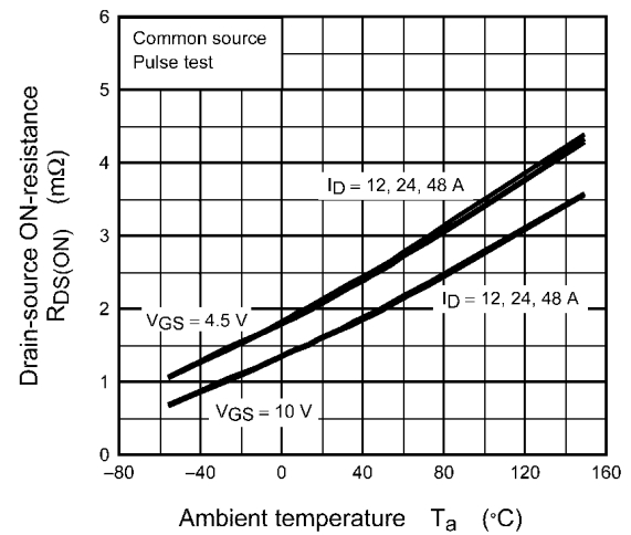
Fig. 8.6 R_{DS(ON)} - T_a
