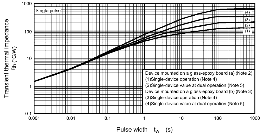
Fig. 8.2.12 r_{th} - t_w (Guaranteed Maximum)
