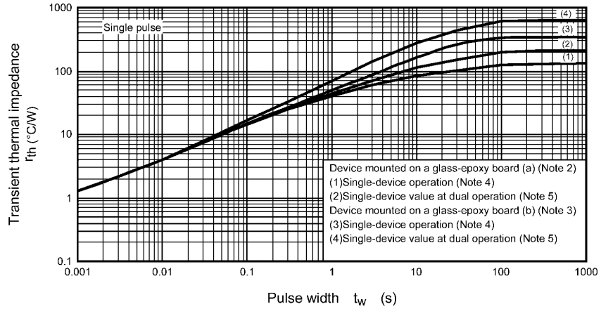
Fig. 8.1.12 r_{th} - t_w (Guaranteed Maximum)
