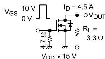
Duty ≤ 1%, t_w = 10\ \mu\text{s}
