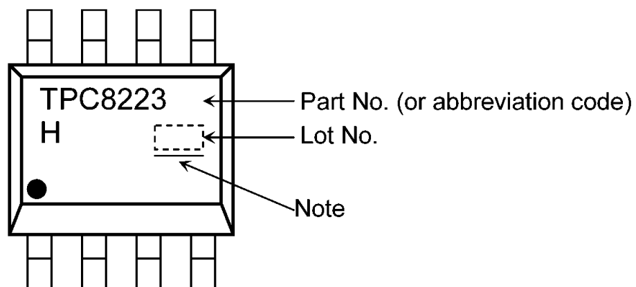
Fig. 7.1 Marking
