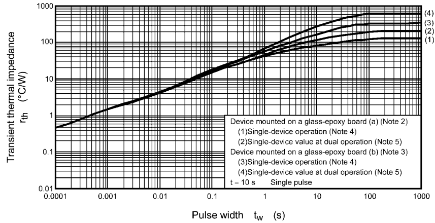
Fig. 8.12 r_{th} - t_w (Guaranteed Maximum)
