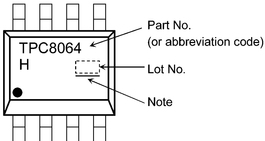
Fig. 7.1 Marking
