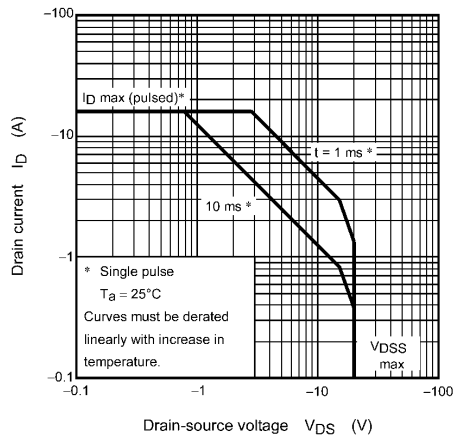
Fig. 8.13 Safe Operating Area (Guaranteed Maximum)
