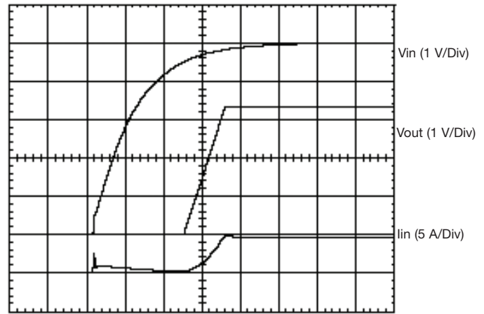
Figure 7 - Power-up Characteristic
