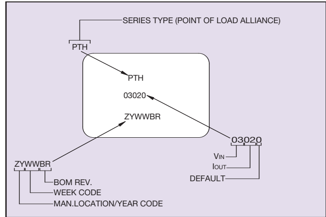
Figure 5 - PTH03020 Part Numbering
