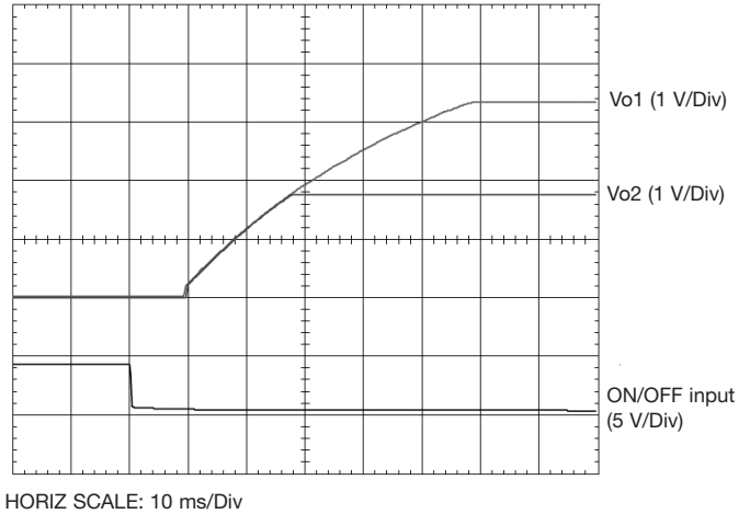
Figure 16 - Power Up with Auto-Track Control
