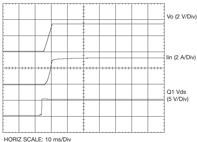
Figure 10 - Typical Rise in Output Voltage and Input Current
