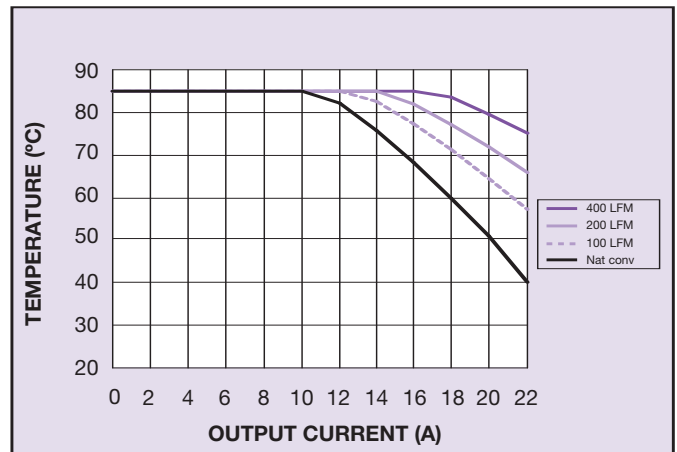
Figure 12 - Safe Operating Curve PTH03020W V_{out} = 2.5 V
