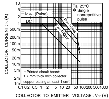
Fig.9 Safe operating area (2SB1241)
