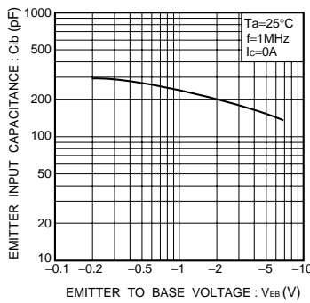
Fig.7 Emitter input capacitance vs. emitter-base voltage
