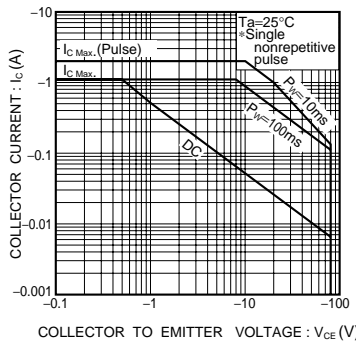
Fig.8 Safe operating area (2SB1260)
