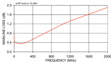
ZFDC-20-5 MAINLINE LOSS
