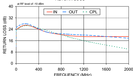
ZFDC-20-5 RETURN LOSS
