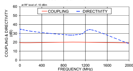
ZFDC-20-5 COUPLING & DIRECTIVITY
