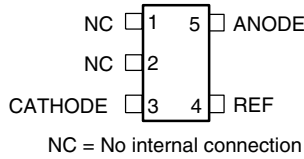
SOT-23 PACKAGE (5-Lead) (TOP VIEW)
