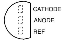
TO-92 PACKAGE (TOP VIEW)
