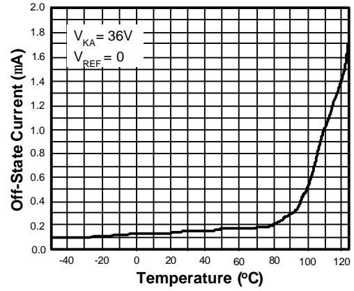
Off-State Current vs. Temperature
