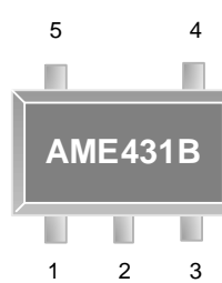
SOT-25/TSOT-25 Top View
