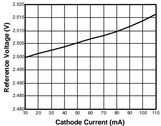
Reference Voltage vs. Cathode Current
