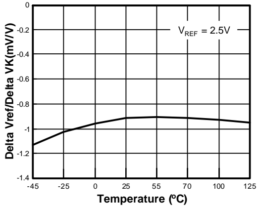
Delta Reference Voltage vs. Temperature
