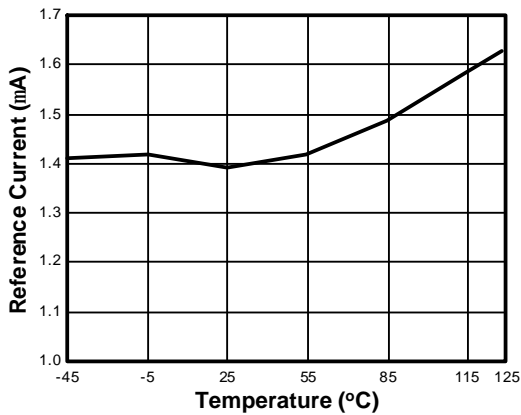
Reference Current vs. Temperature
