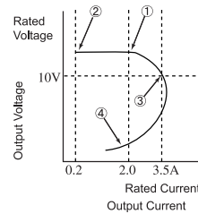
Fig2. Output Voltage/Current
