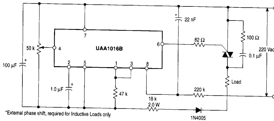
Figure 8. Electronic Rheostat
