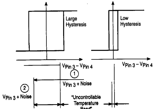
Figure 5. Effects of Inputs Comparator Hysteresis
