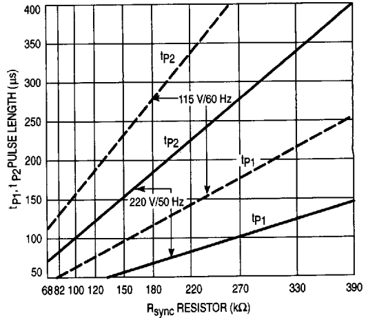
Figure 4. Typical Output Pulse Length versus Synchronization Resistor
