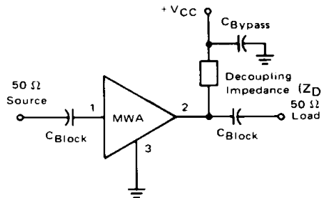
FIGURE 27 – AMPLIFIER SCHEMATIC DIAGRAM
