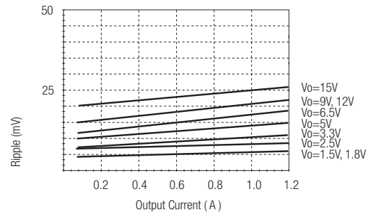
Ripple Vs Load (Vin=Max)
