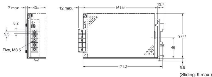
S82J-050□□□D (50 W)
