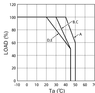
Convection Cooling Output Derating Curve (With cover)
