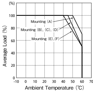
ZWS50AF Output Derating
