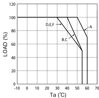
Convection Cooling Output Derating Curve (Without cover)
