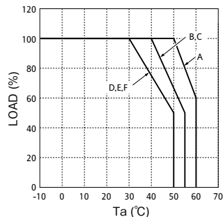
Convection Cooling Output Derating Curve (Without cover)
