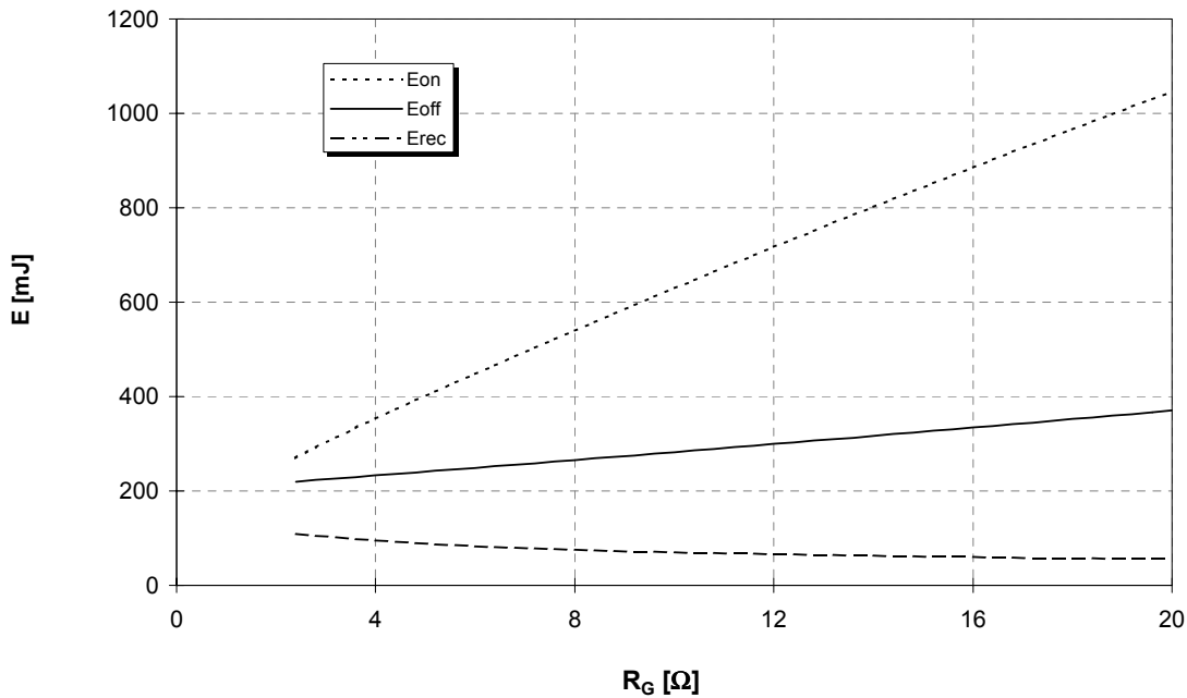
Schaltverluste (typisch) E_{on} = f(R_G) , E_{off} = f(R_G) , E_{rec} = f(R_G) Switching losses (typical) I_C = 600A , V_{CE} = 900V , T_j = 125^\circ C
