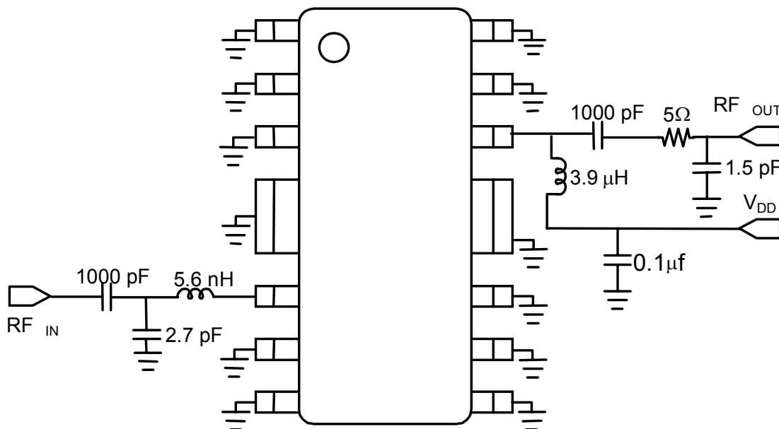
Figure 3: Test Circuit
