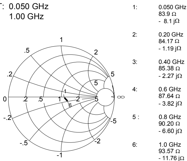
Figure 9: Output Impedance
