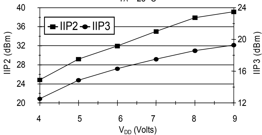
Figure 6: IIP2, IIP3 vs. VDD
