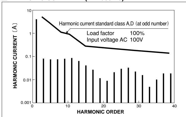
HARMONIC CURRENT (PAA300F-5)
