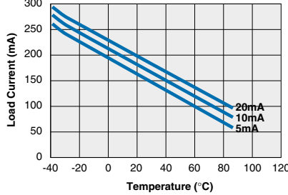
PAA110 Typical Load Current vs. Temperature
