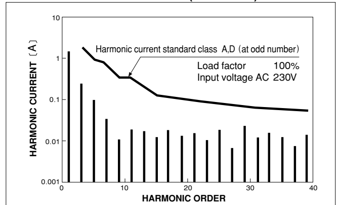
INPUT HARMONIC CURRENT (PAA300F-5)
