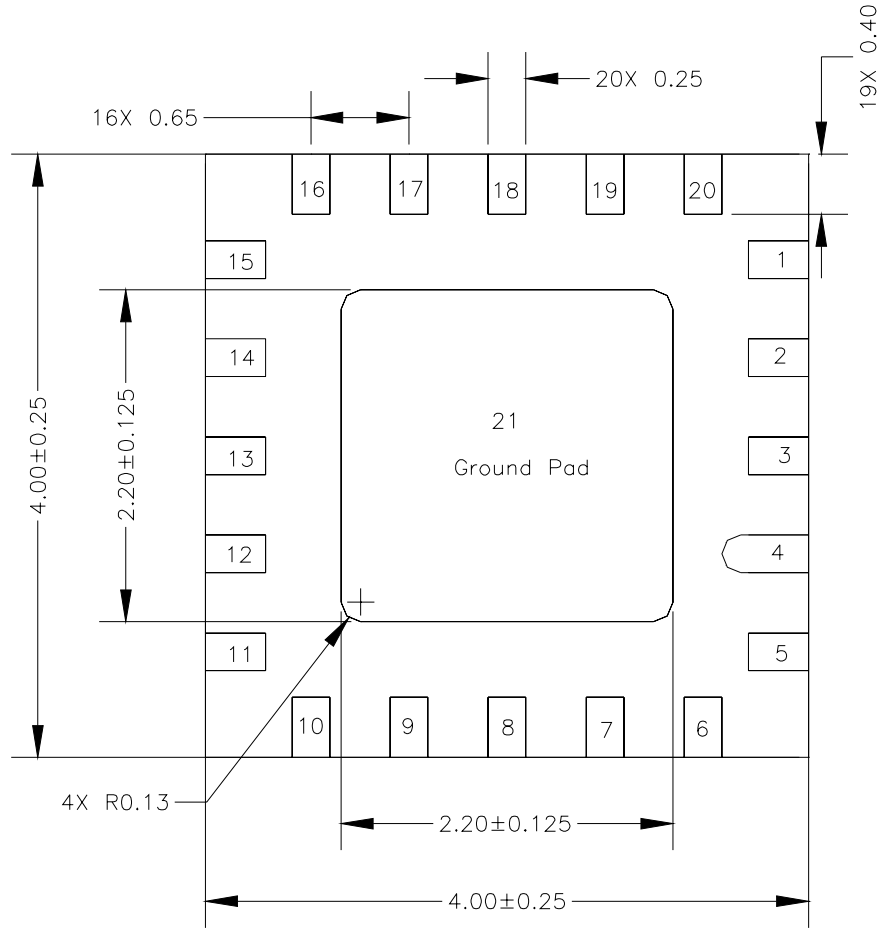
BOTTOM VIEW
