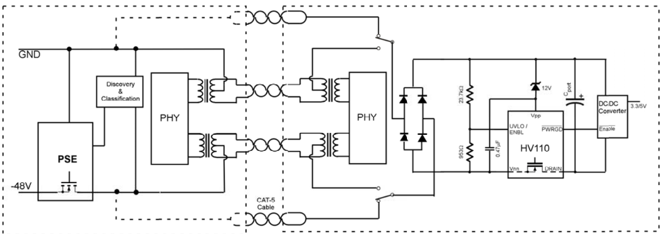
Note: A decoupling capacitor may be connected across VPP and VNN pins when used with long CAT-5 cables
